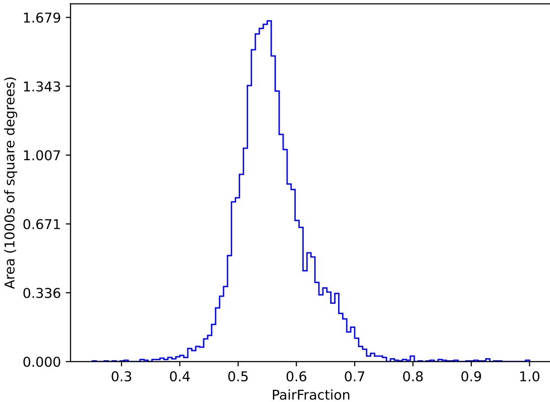
too_10_4v3.4_10yrs (g or r or i): PairFraction
