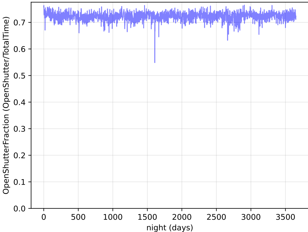
too_10_4v3.4_10yrs : OpenShutterFraction
