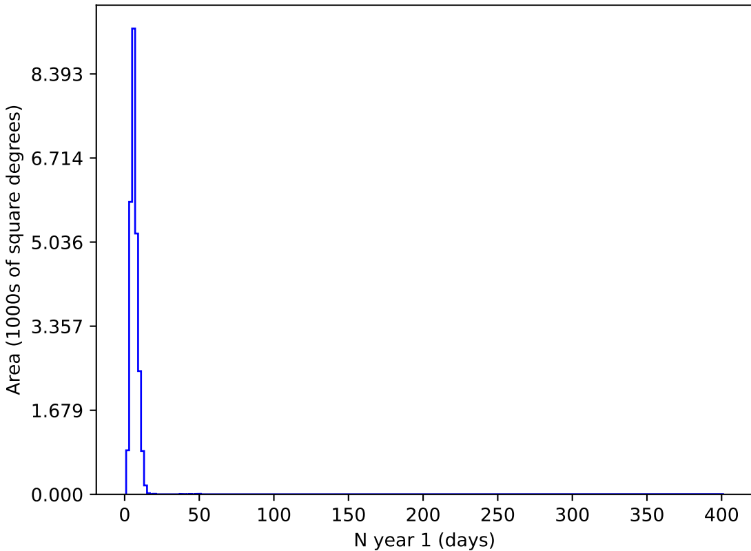
too_10_4v3.4_10yrs u and night < 365: N year 1
