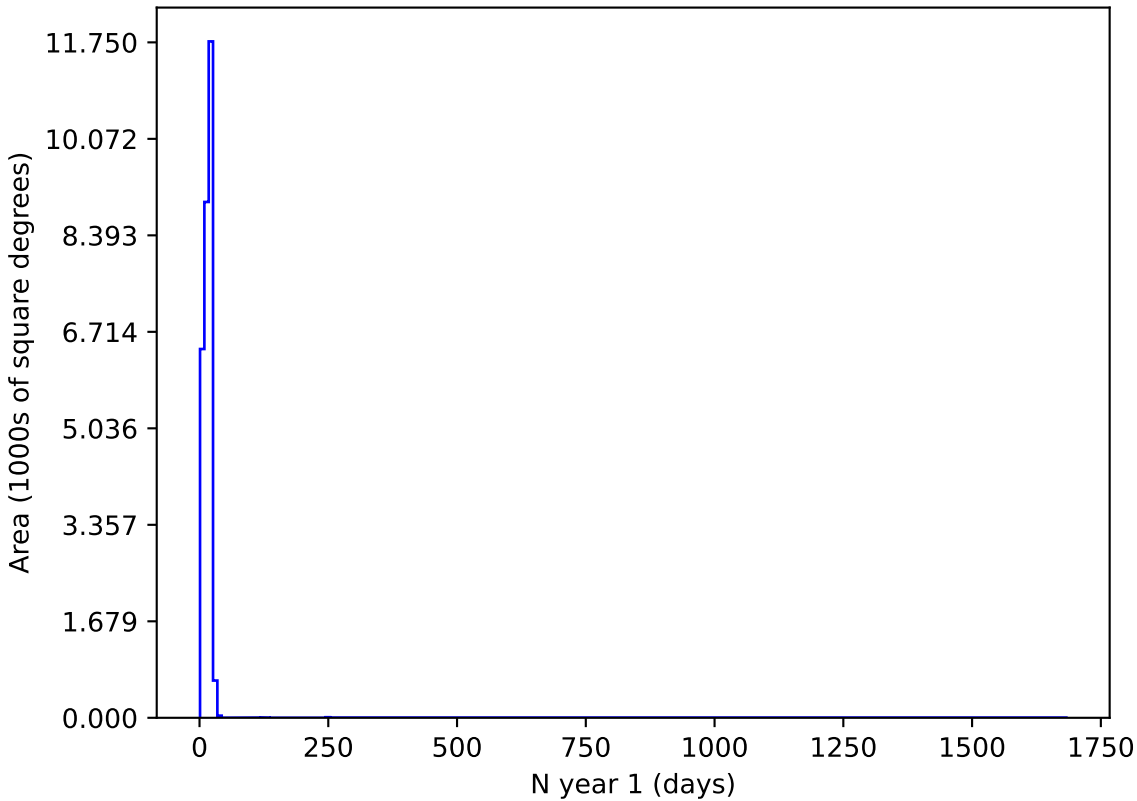
too_10_4v3.4_10yrs r and night < 365: N year 1
