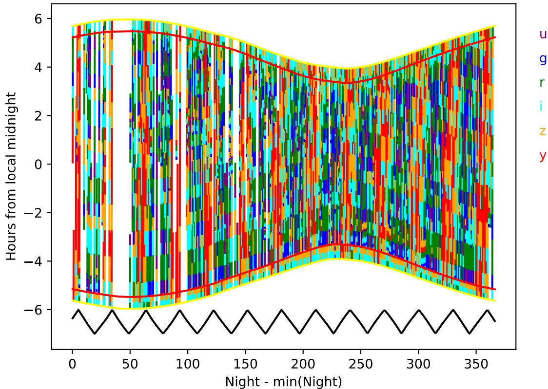
too_10_4v3.4_10yrs year 6-7: Hourglass
