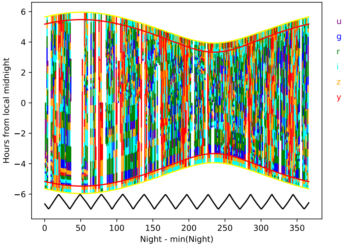
too_10_4v3.4_10yrs year 2-3: Hourglass
