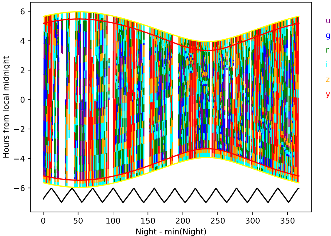
too_10_4v3.4_10yrs year 0-1: Hourglass
