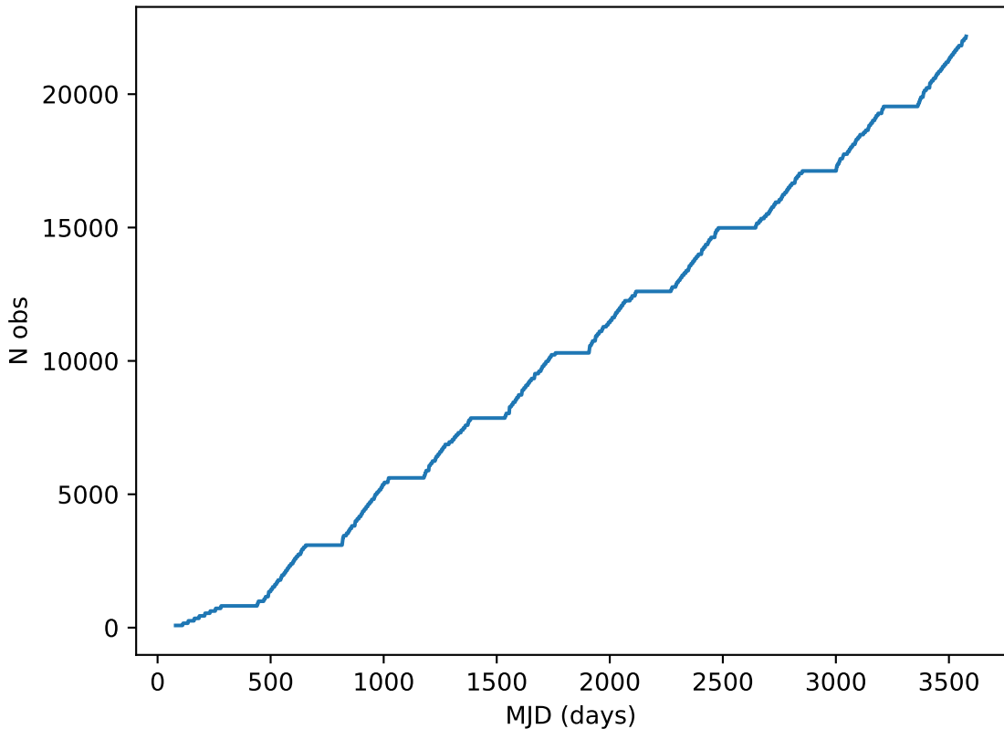
too_10_4v3.4_10yrs note like DD:XMM_LSS%: Cumulative
