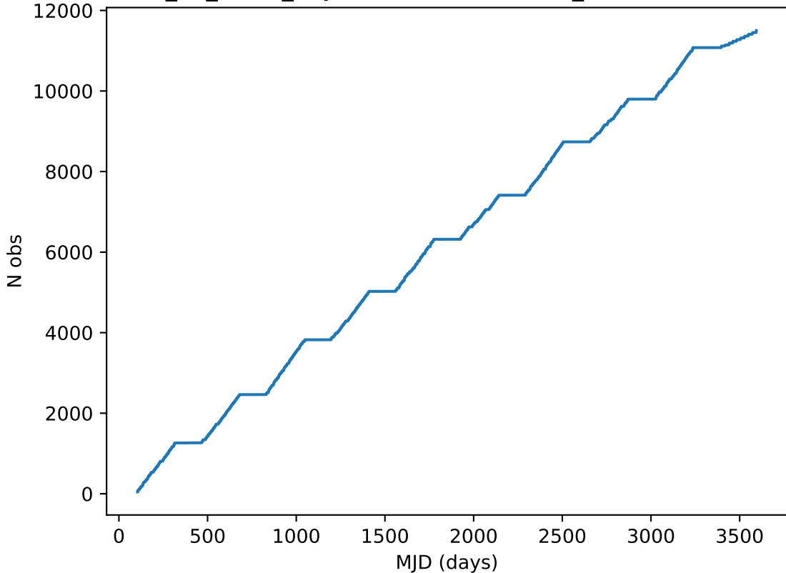
too_10_4v3.4_10yrs note like DD:EDFS_a%: Cumulative
