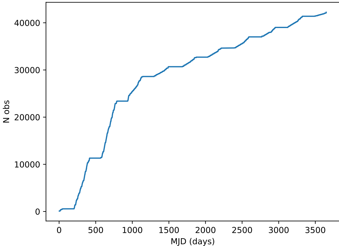
too_10_4v3.4_10yrs note like DD:COSMOS%: Cumulative
