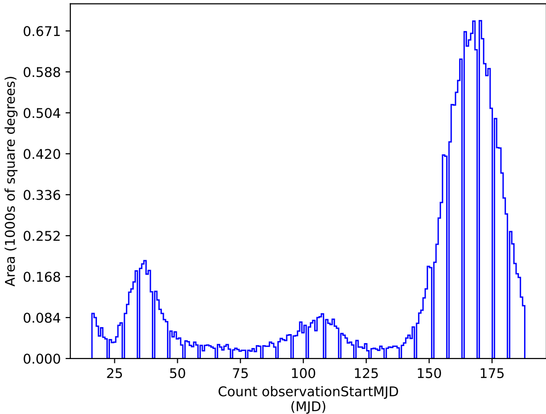
too_10_4v3.4_10yrs y: Count observationStartMJD
