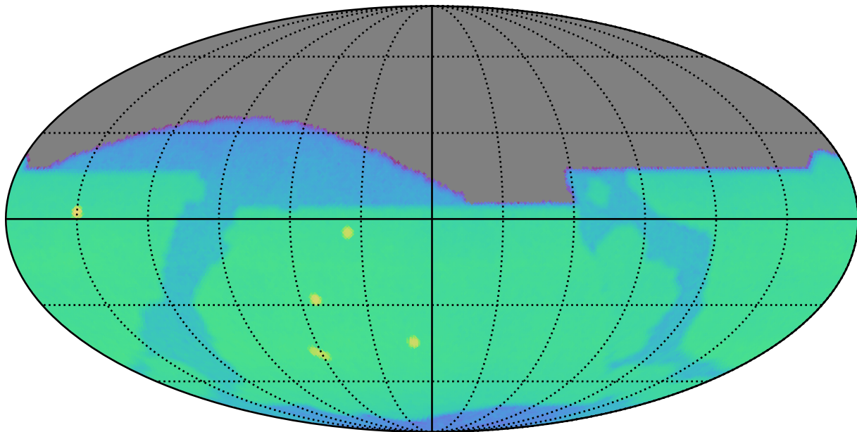
too_10_4v3.4_10yrs z: CoaddM5
