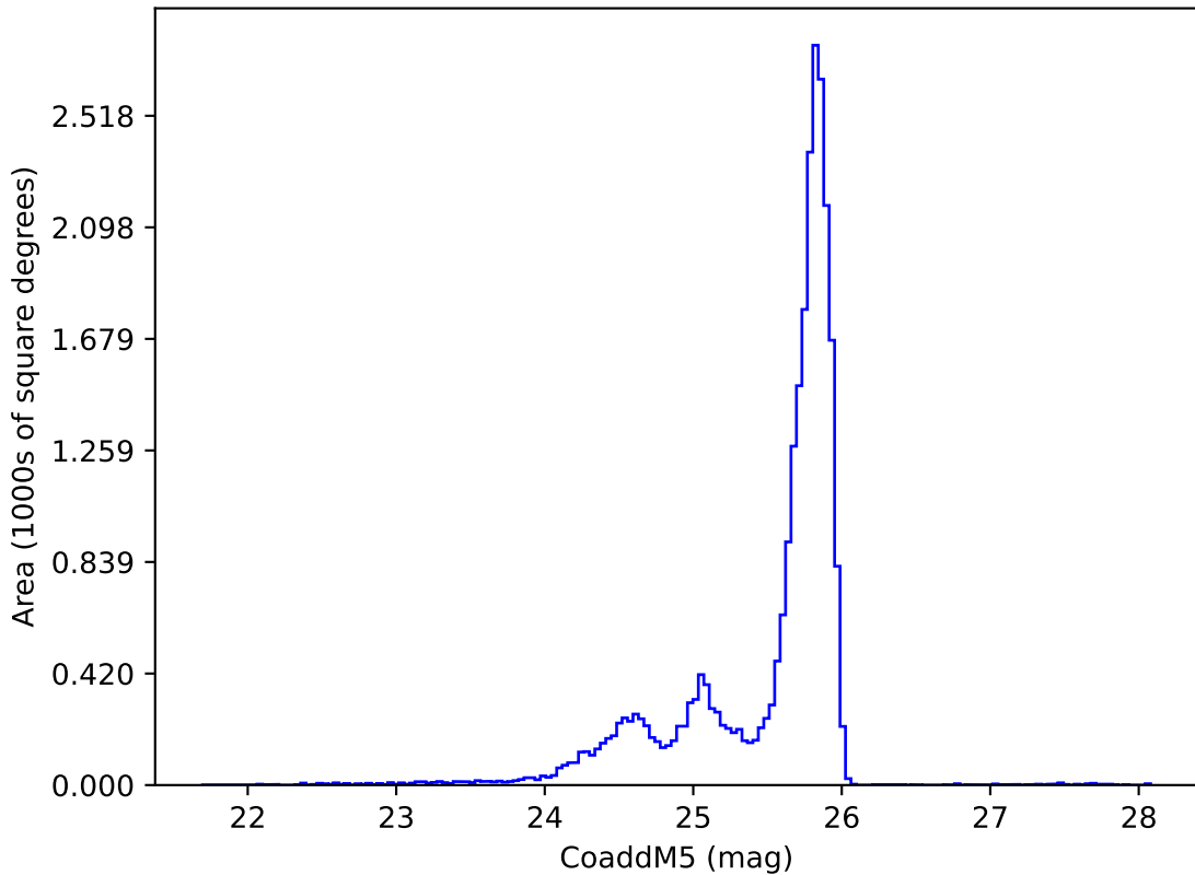
too_10_4v3.4_10yrs z: CoaddM5
