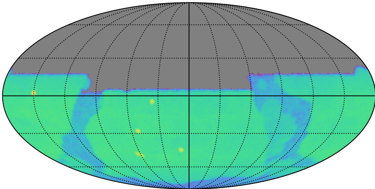
too_10_4v3.4_10yrs u: CoaddM5
