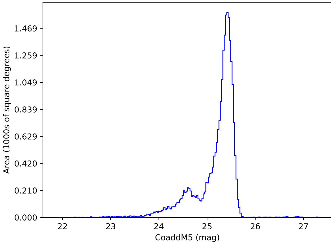
too_10_4v3.4_10yrs u: CoaddM5
