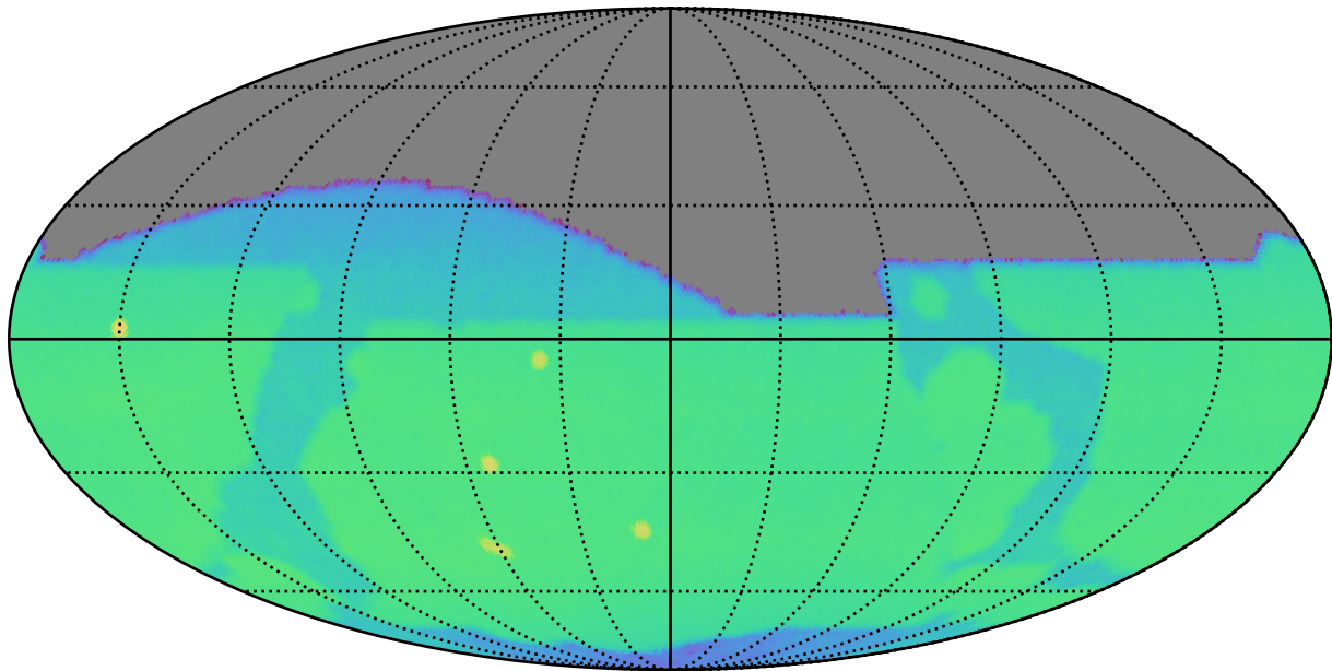
too_10_4v3.4_10yrs r: CoaddM5
