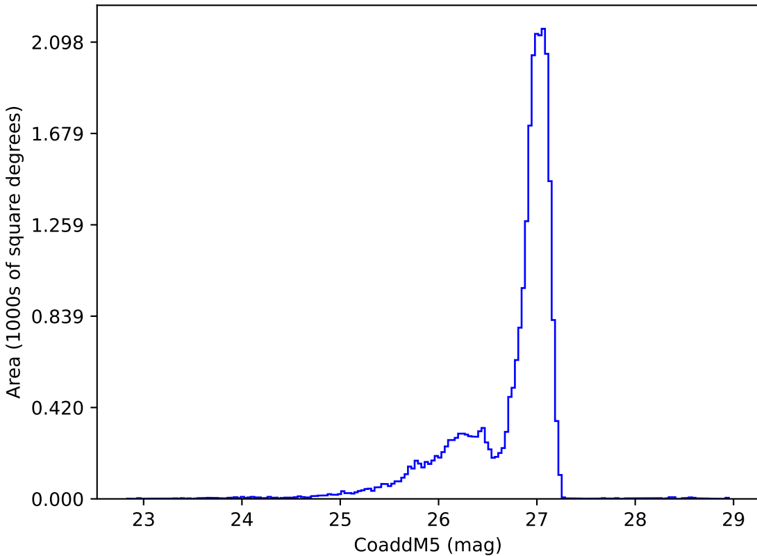
too_10_4v3.4_10yrs r: CoaddM5
