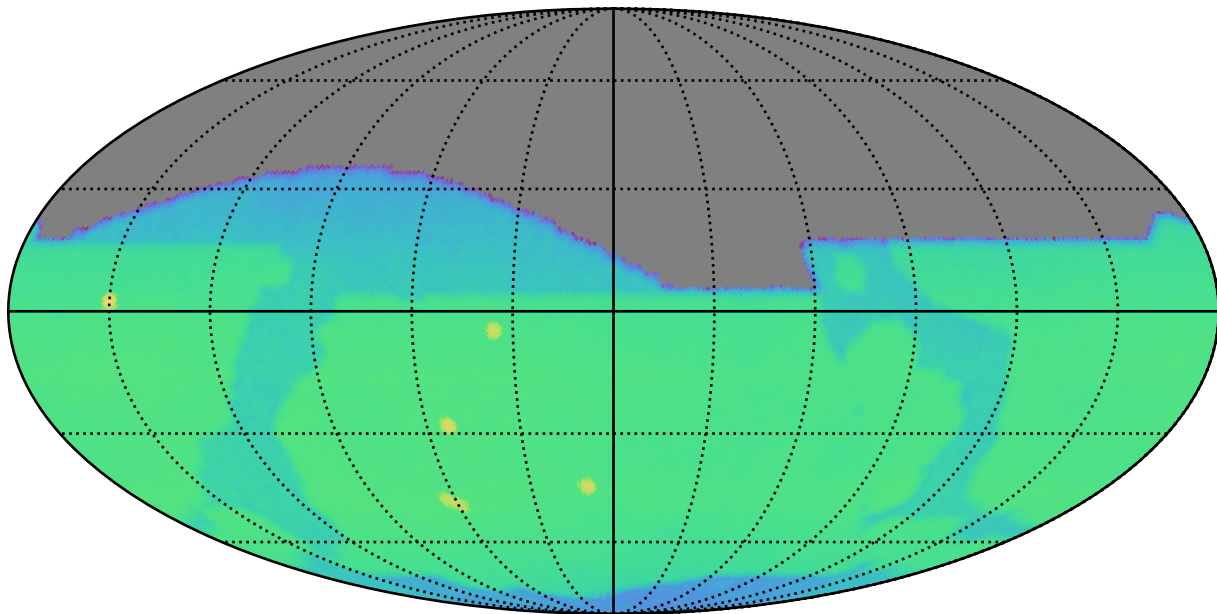
too_10_4v3.4_10yrs i: CoaddM5
