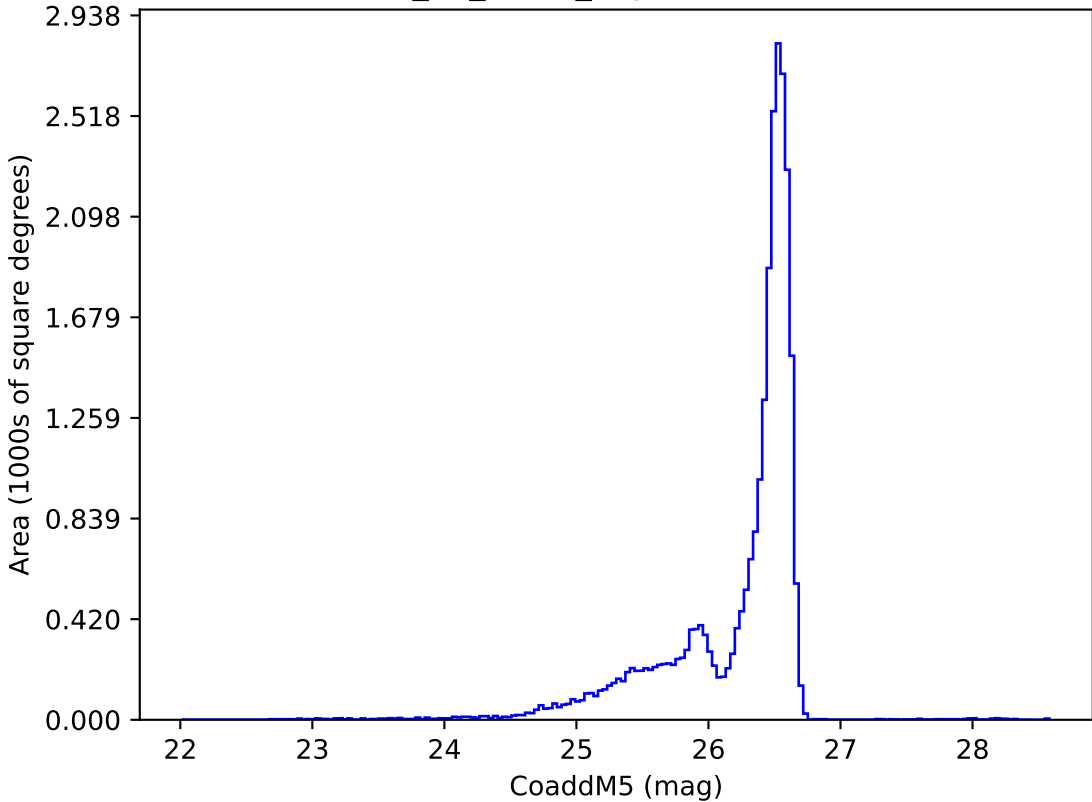
too_10_4v3.4_10yrs i: CoaddM5
