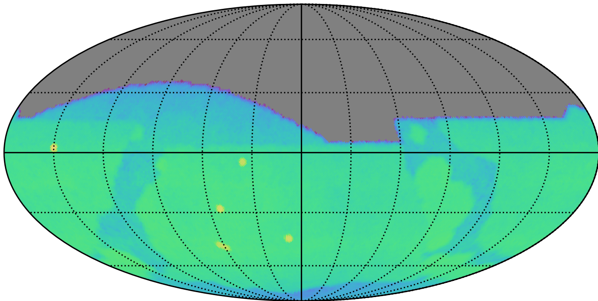
too_10_4v3.4_10yrs g: CoaddM5
