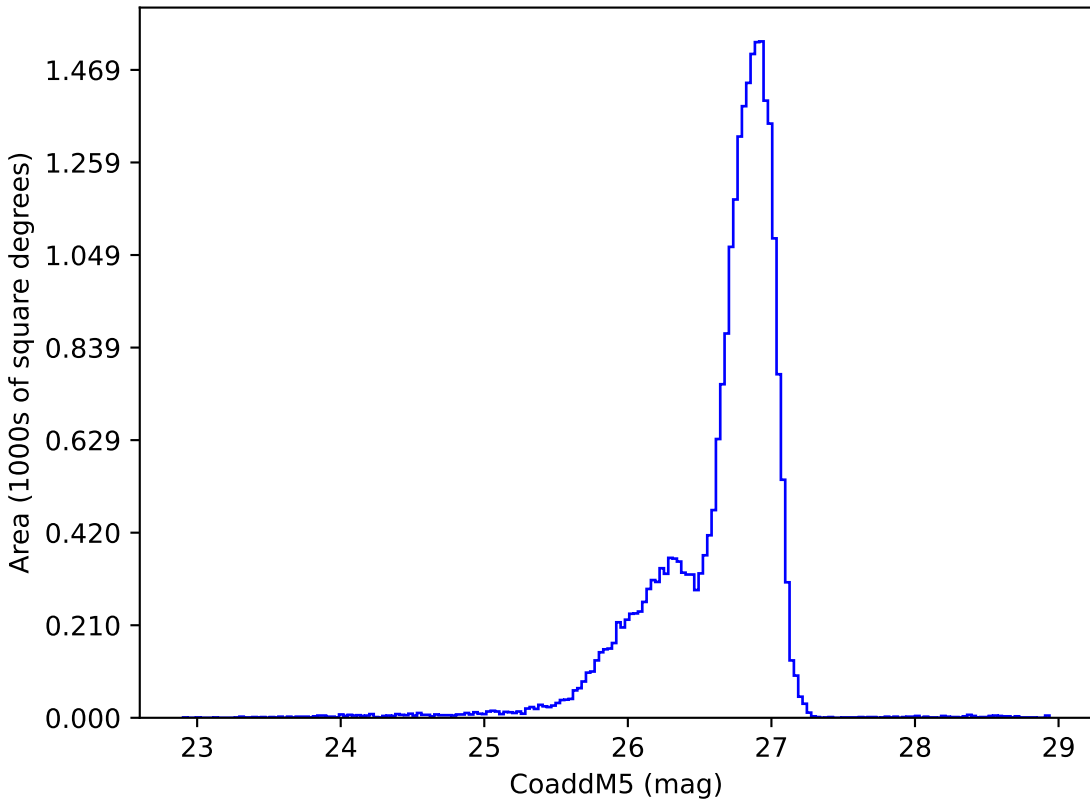
too_10_4v3.4_10yrs g: CoaddM5
