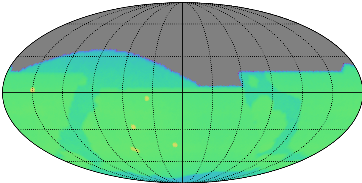
too_10_4v3.4_10yrs : CoaddM5
