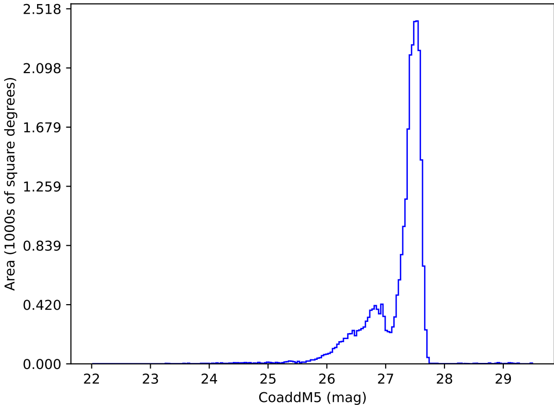
too_10_4v3.4_10yrs : CoaddM5
