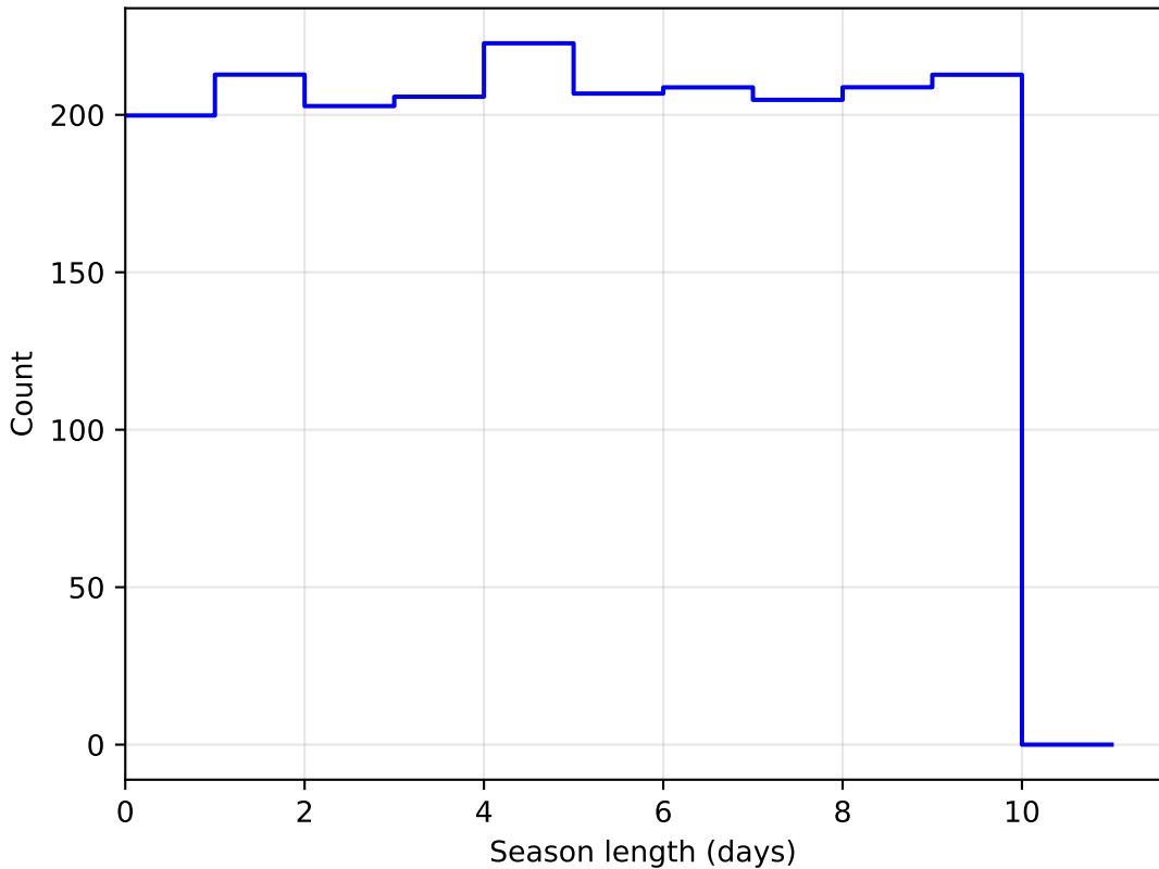
too_10_4v3.4_10yrs DD:XMM_LSS all bands: SeasonLength
