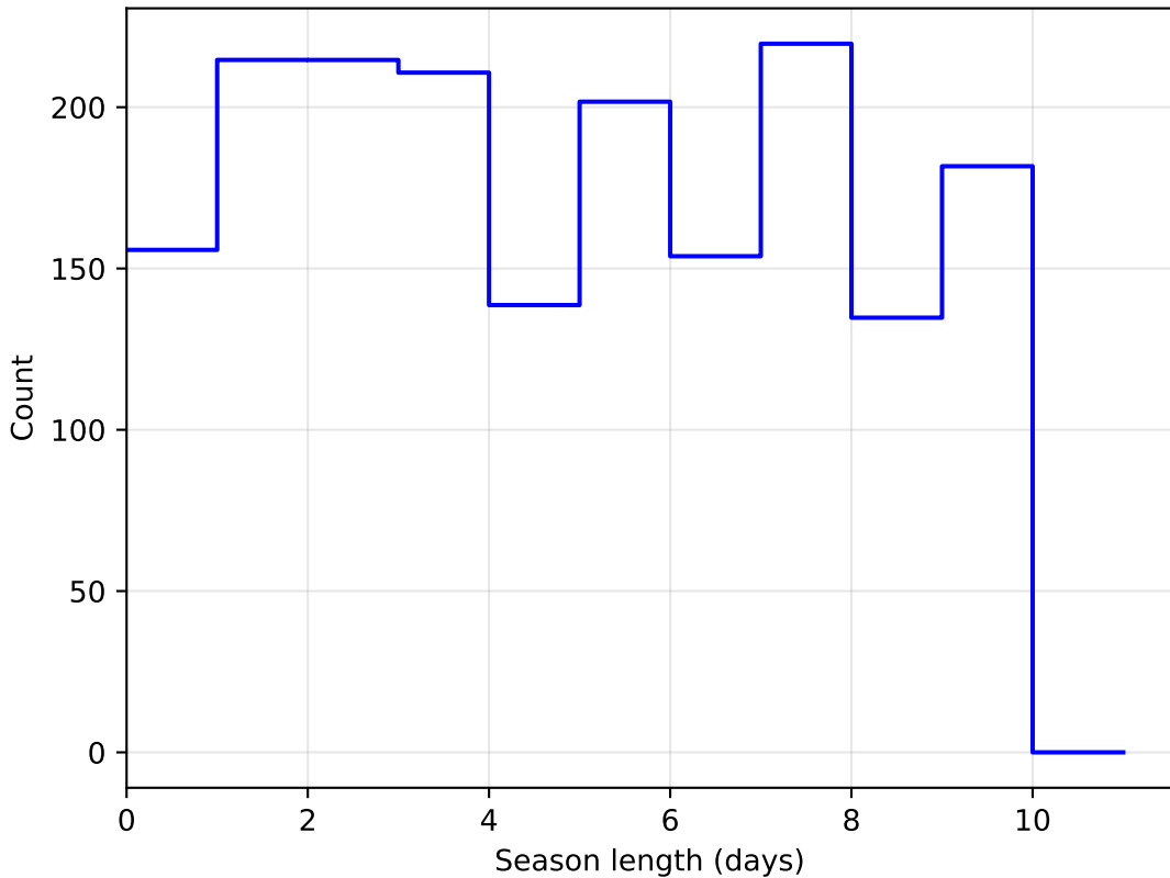
too_10_4v3.4_10yrs DD:WFD all bands: SeasonLength
