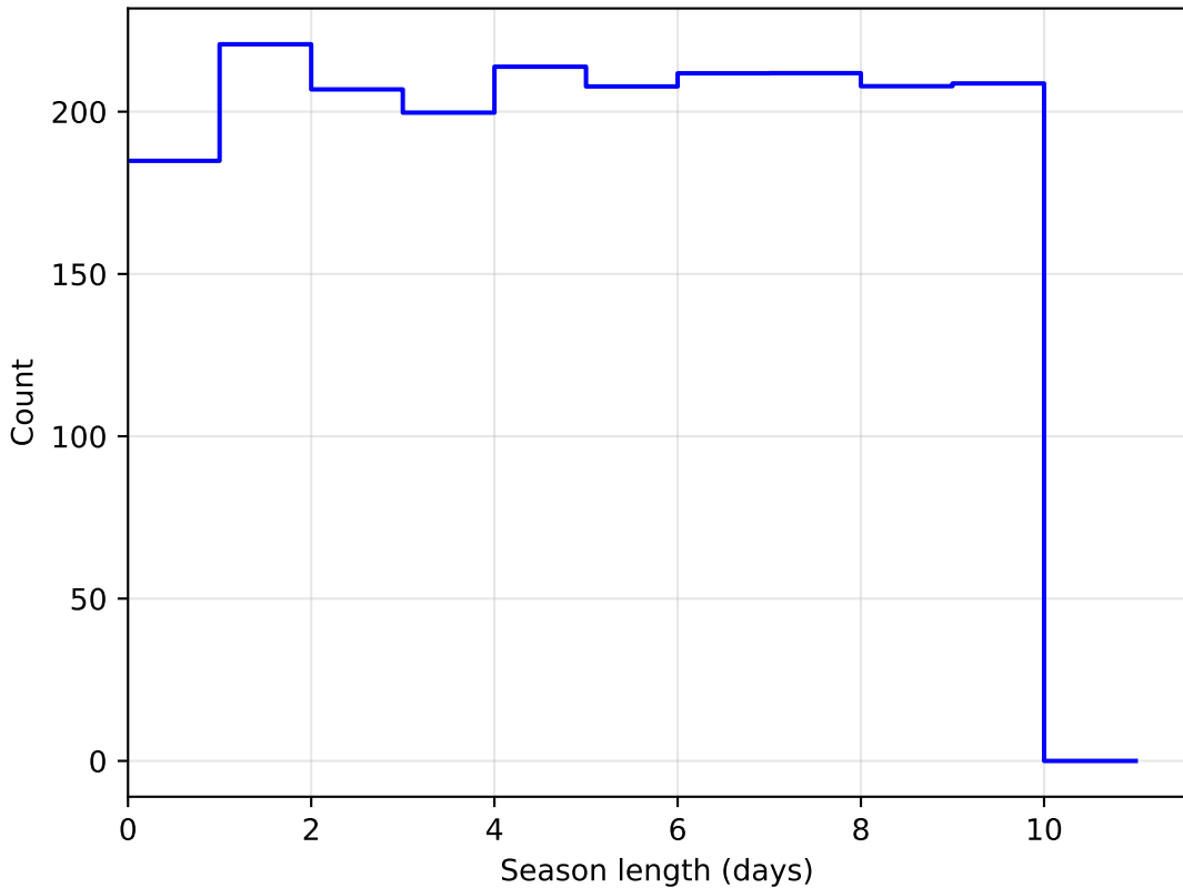
too_10_4v3.4_10yrs DD:ELAISS1 all bands: SeasonLength
