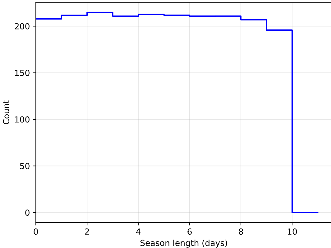
too_10_4v3.4_10yrs DD:EDFS all bands: SeasonLength
