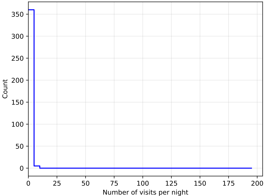
too_10_4v3.4_10yrs all bands: DD:WFD NVisitsPerNight
