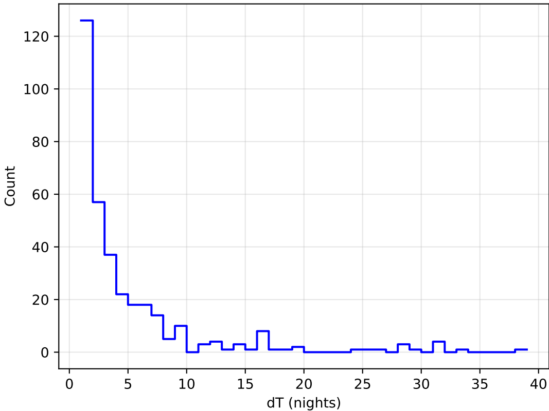
too_10_4v3.4_10yrs all bands: DD:WFD Delta Nights Histogram
