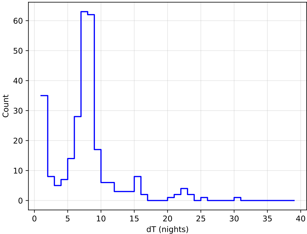
too_10_4v3.4_10yrs all bands: DD:ECDFS Delta Nights Histogram
