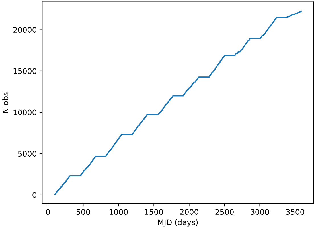
too_10_4v3.4_10yrs all bands: DD:ECDFS Cumulative NVisits
