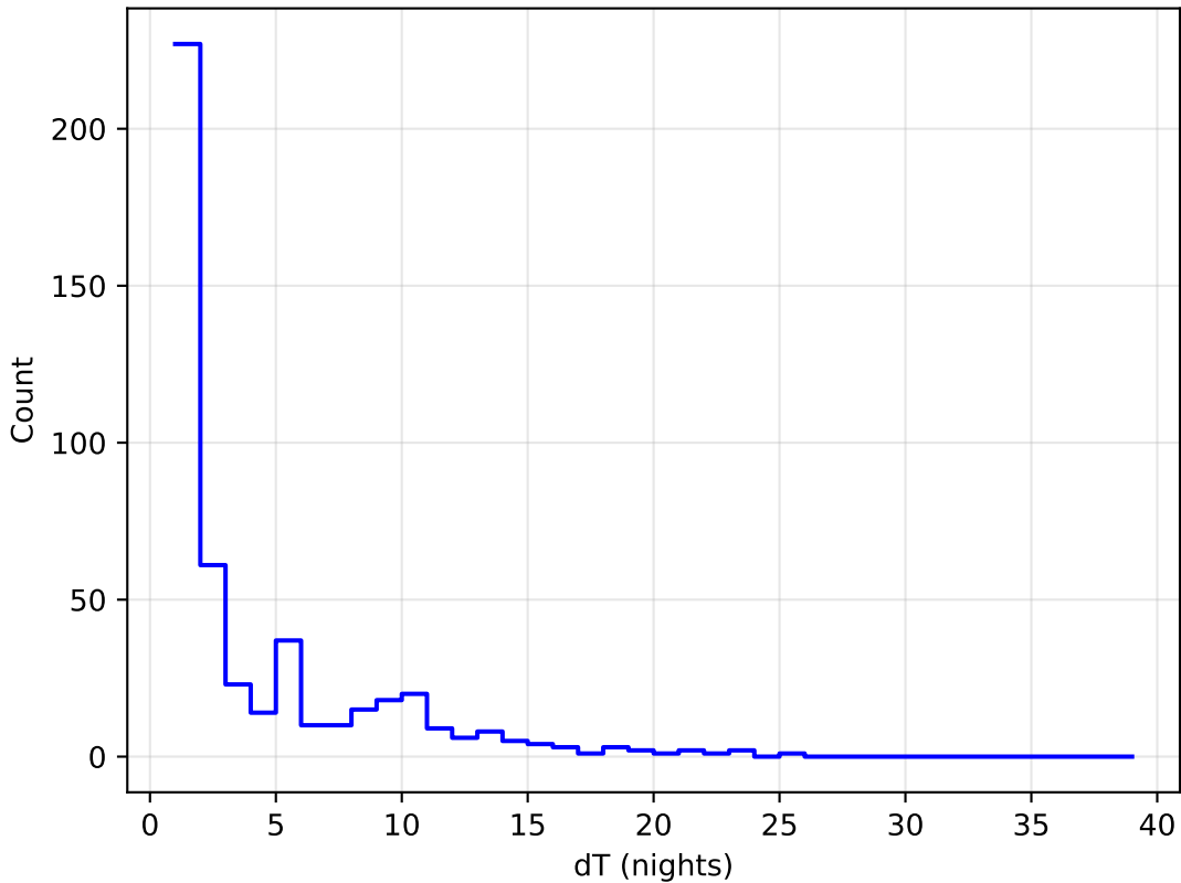
too_10_4v3.4_10yrs all bands: DD: COSMOS Delta Nights Histogram
