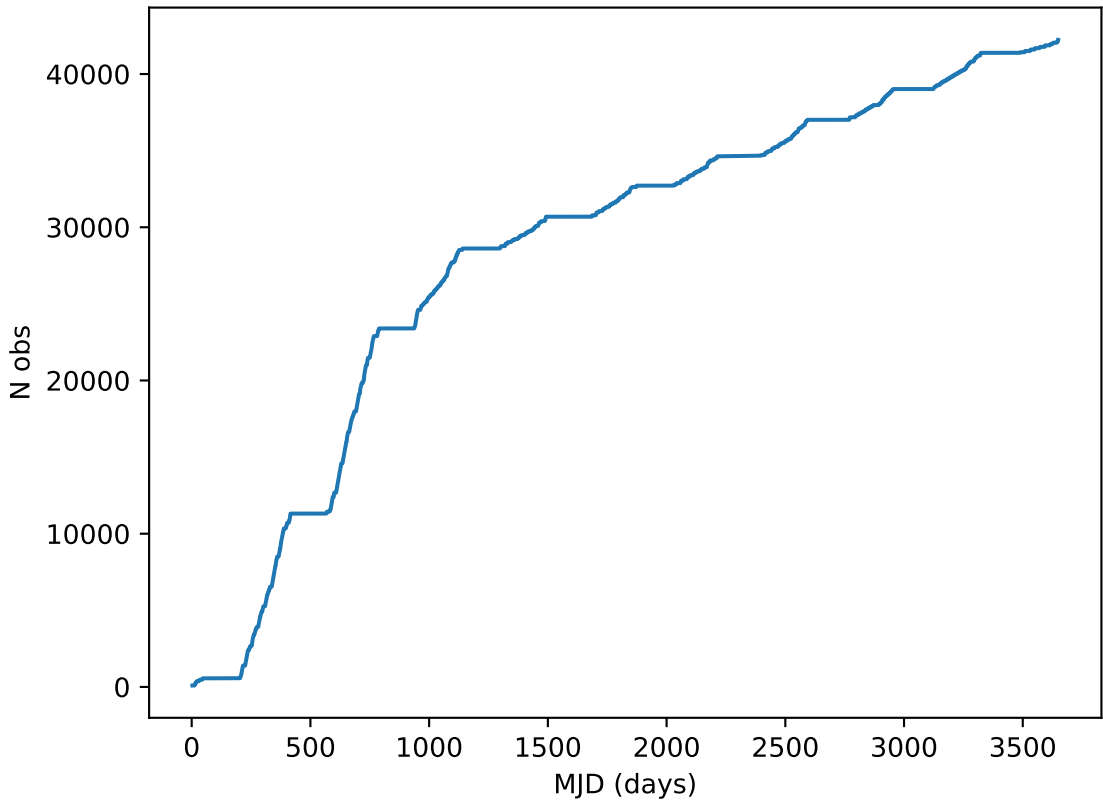
too_10_4v3.4_10yrs all bands: DD:COSMOS Cumulative NVisits
