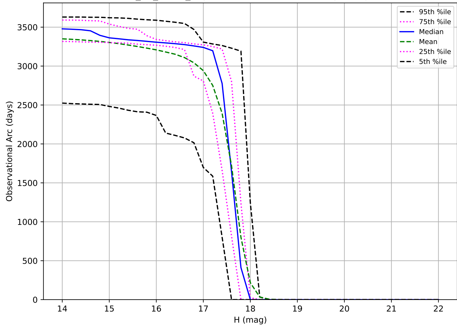
too_10_1v3.4_10yrs: Observational Arc Length Trojan
