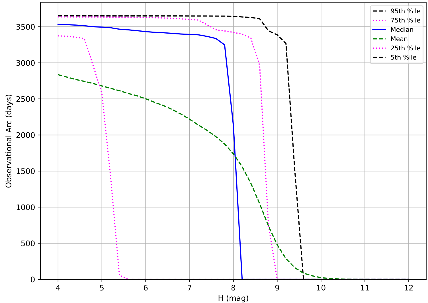
too_10_1v3.4_10yrs: Observational Arc Length TNO
