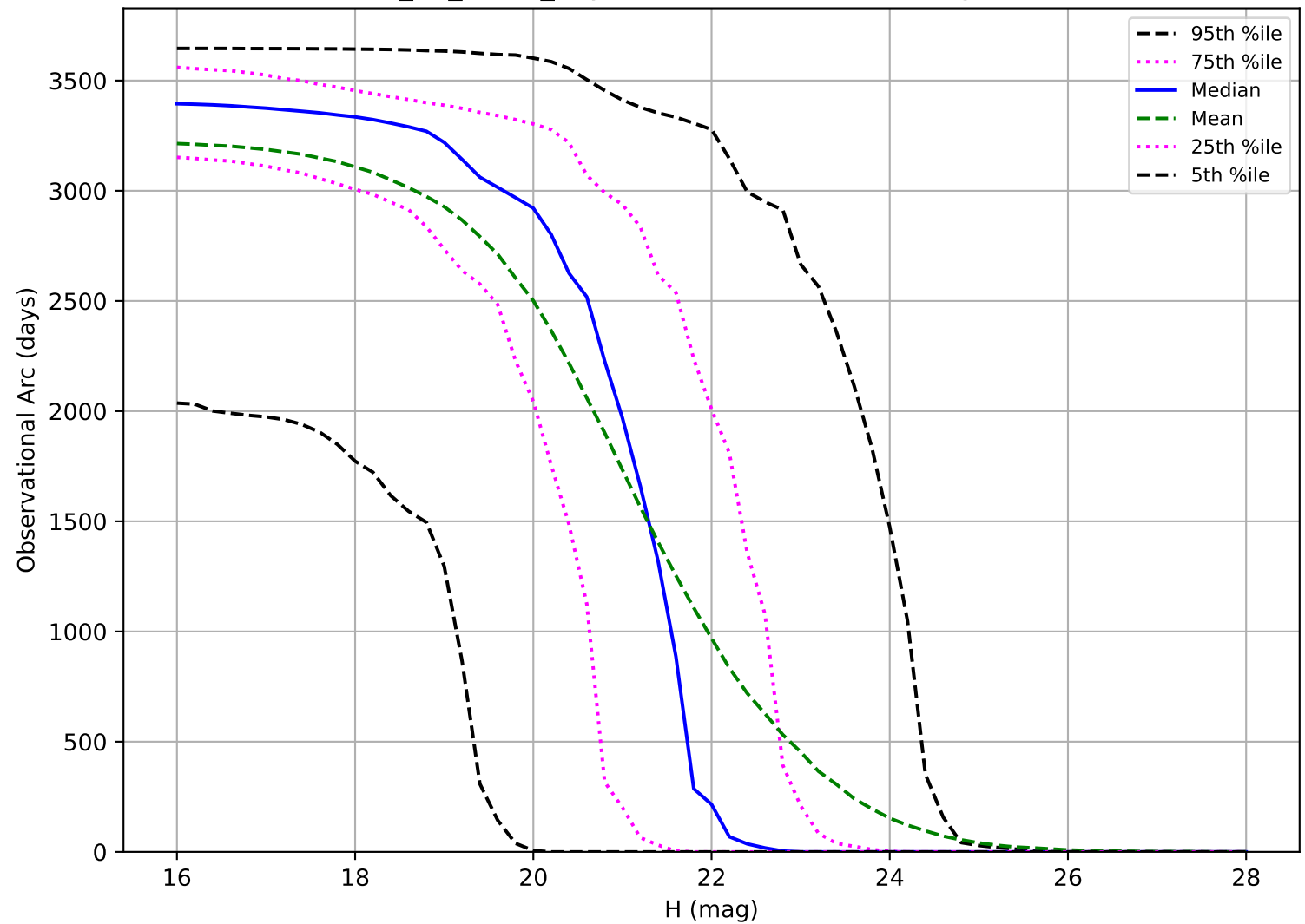
too_10_1v3.4_10yrs: Observational Arc Length PHA
