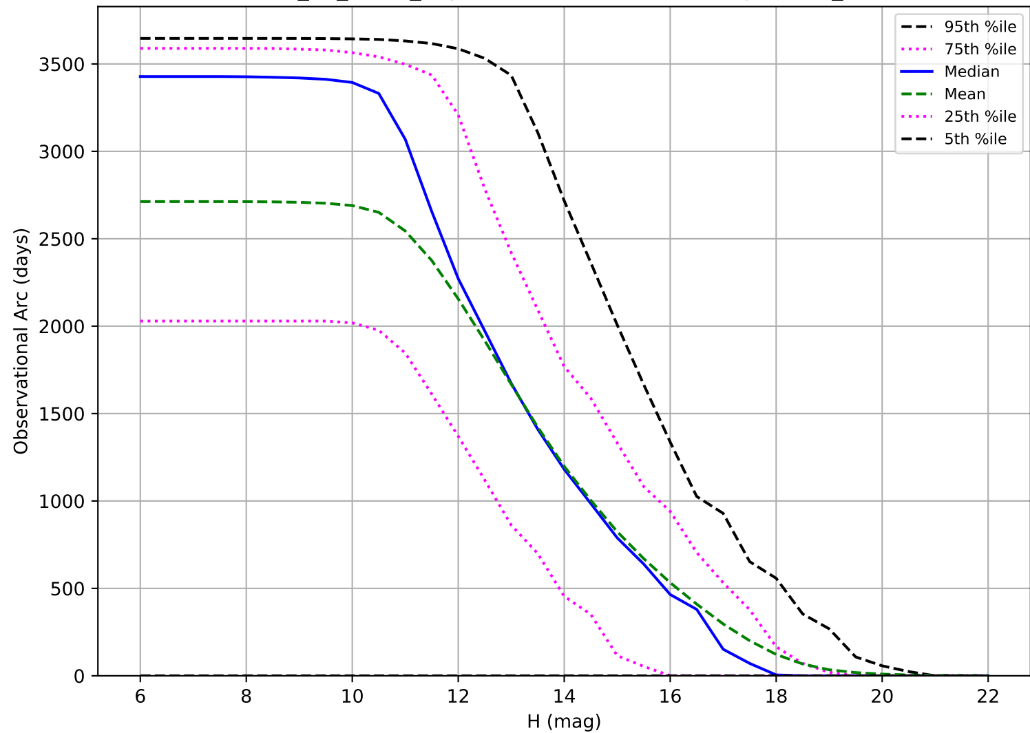
too_10_1v3.4_10yrs: Observational Arc Length OCC_r5
