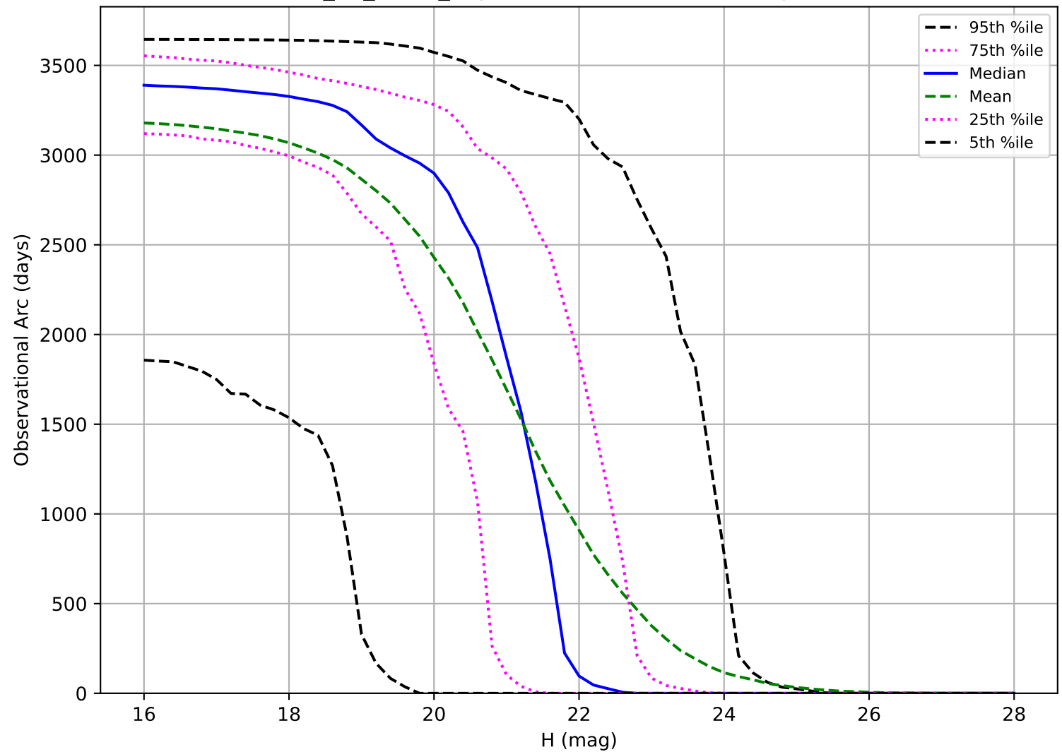
too_10_1v3.4_10yrs: Observational Arc Length NEO
