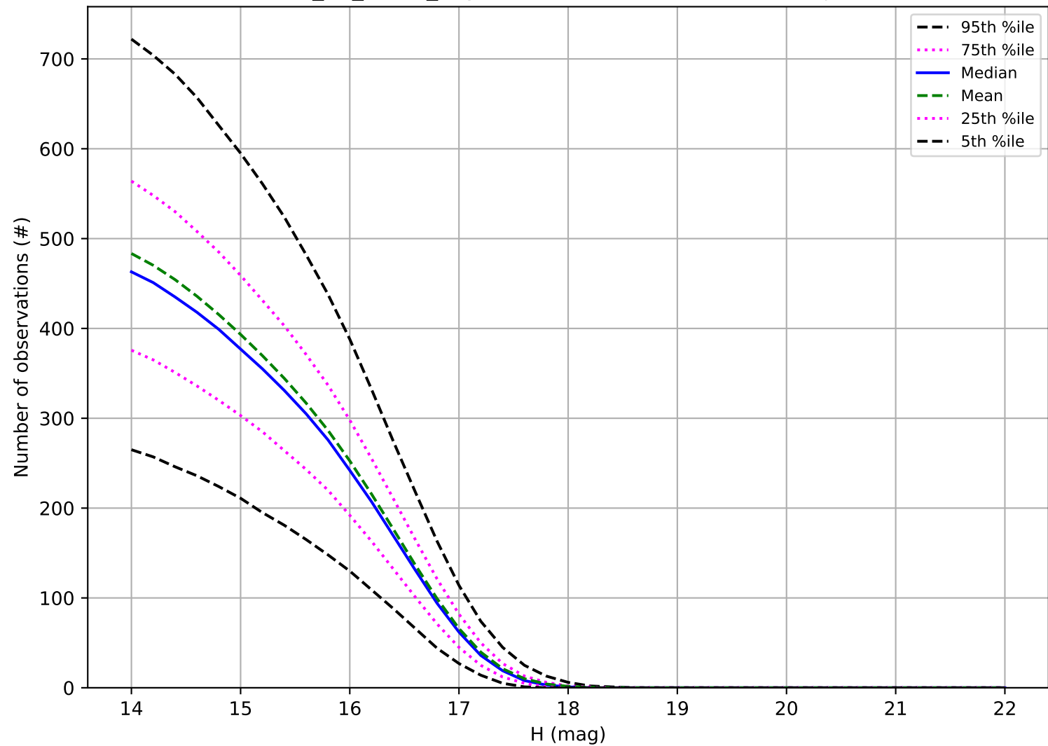
too_10_1v3.4_10yrs: Number of observations Trojan
