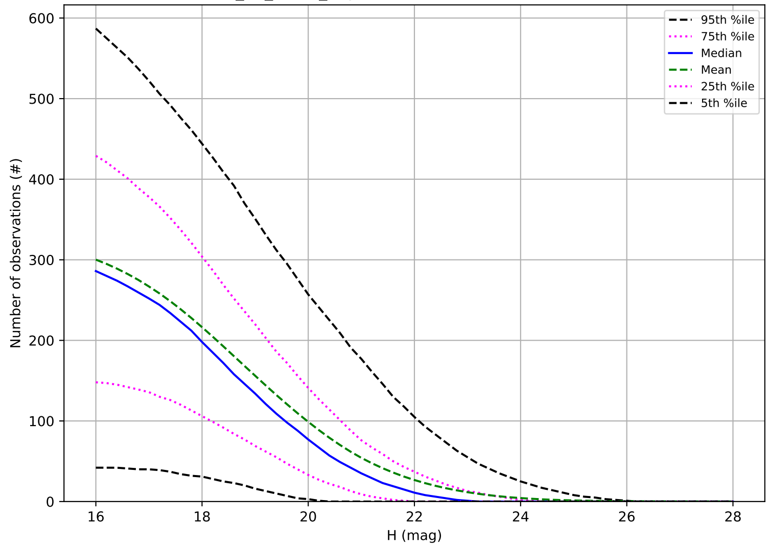
too_10_1v3.4_10yrs: Number of observations PHA
