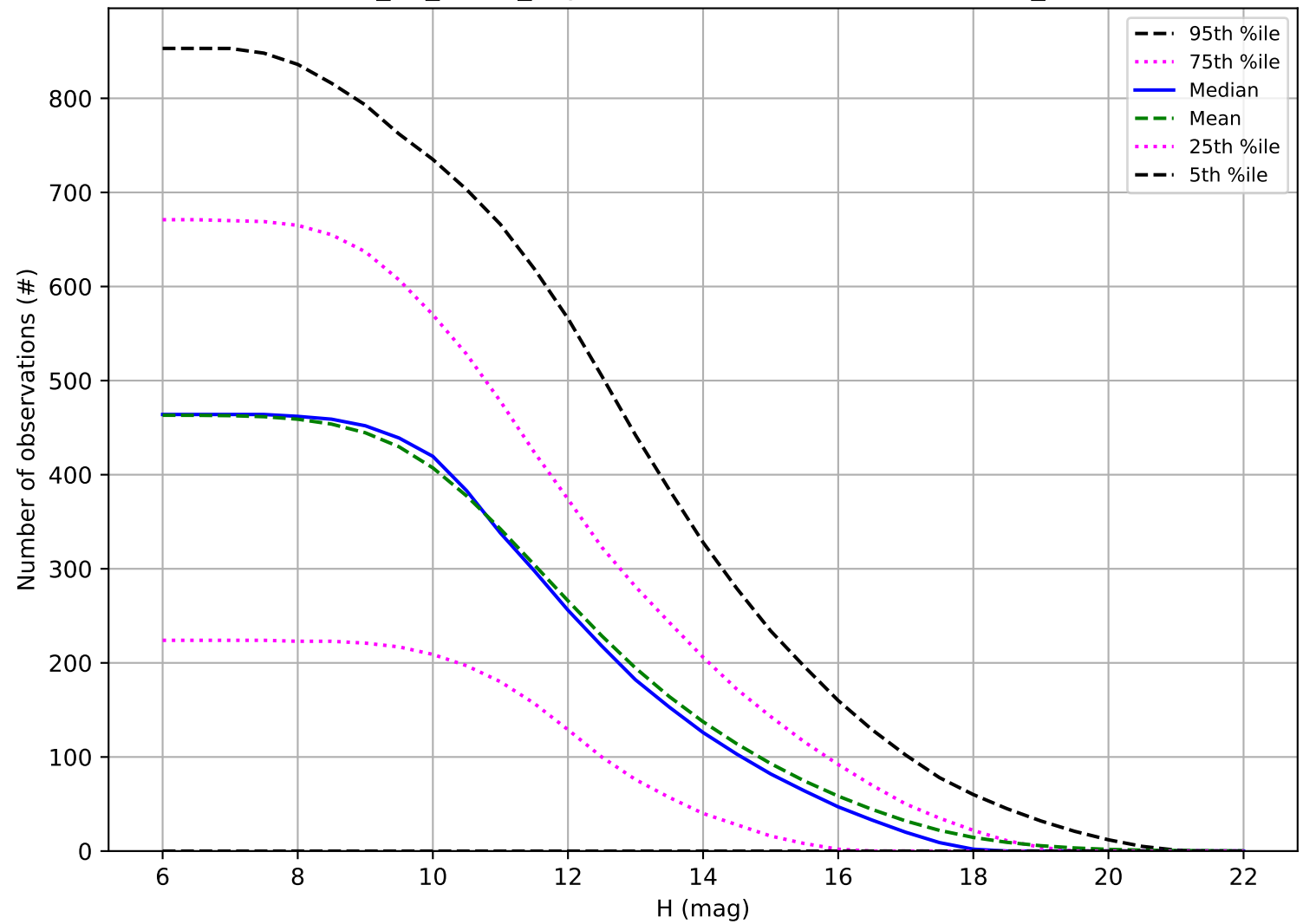
too_10_1v3.4_10yrs: Number of observations OCC_r5
