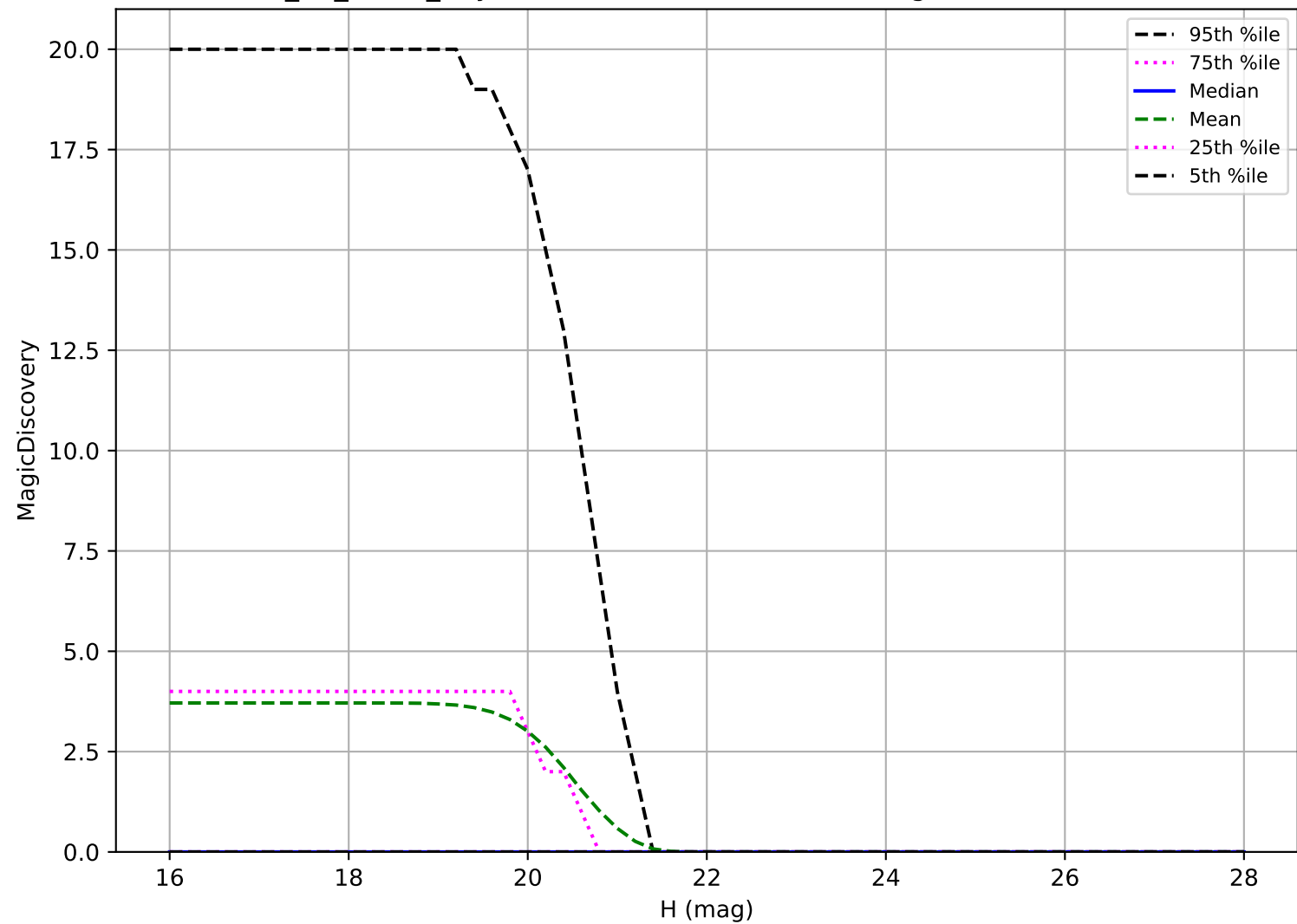
too_10_1v3.4_10yrs: Vatira 6 detections in 60 nights detection loss
