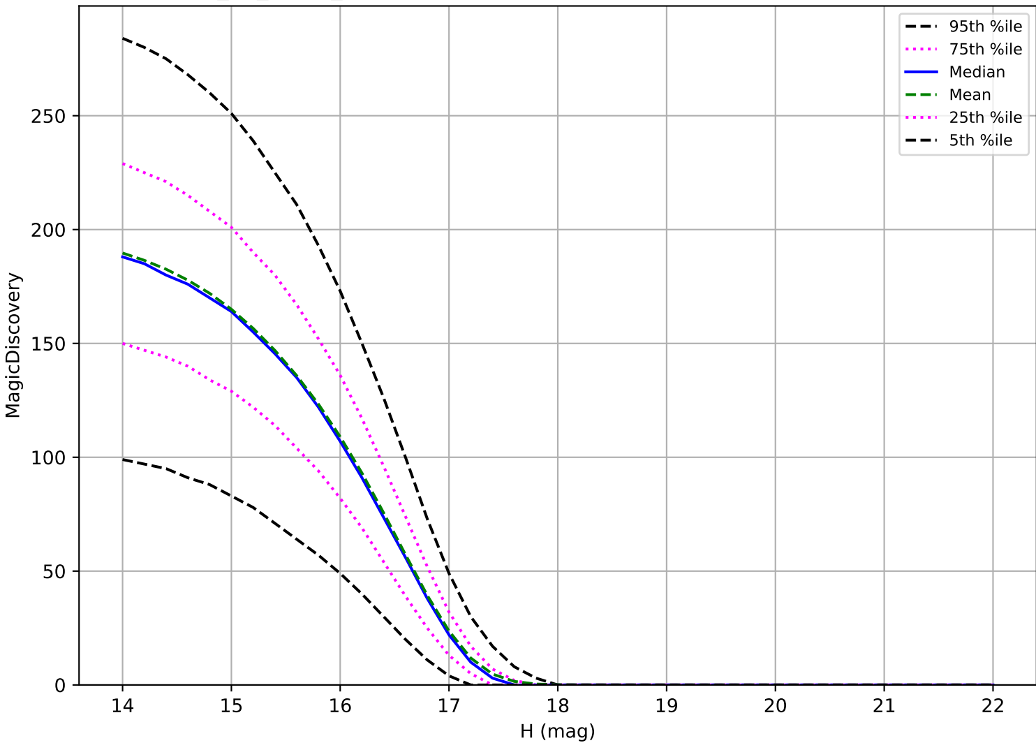
too_10_1v3.4_10yrs: Trojan 6 detections in 60 nights detection loss
