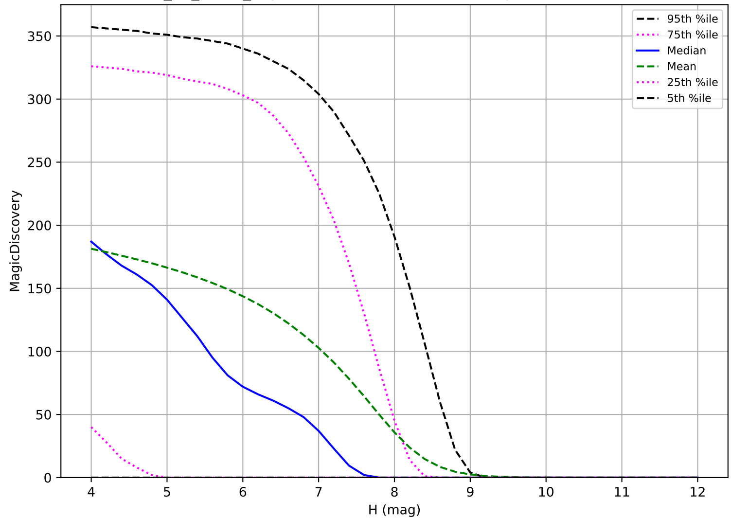
too_10_1v3.4_10yrs: TNO 6 detections in 60 nights detection loss
