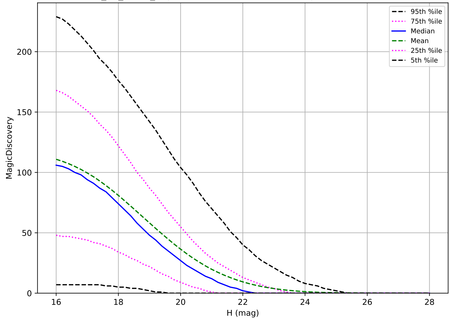
too_10_1v3.4_10yrs: PHA 6 detections in 60 nights detection loss
