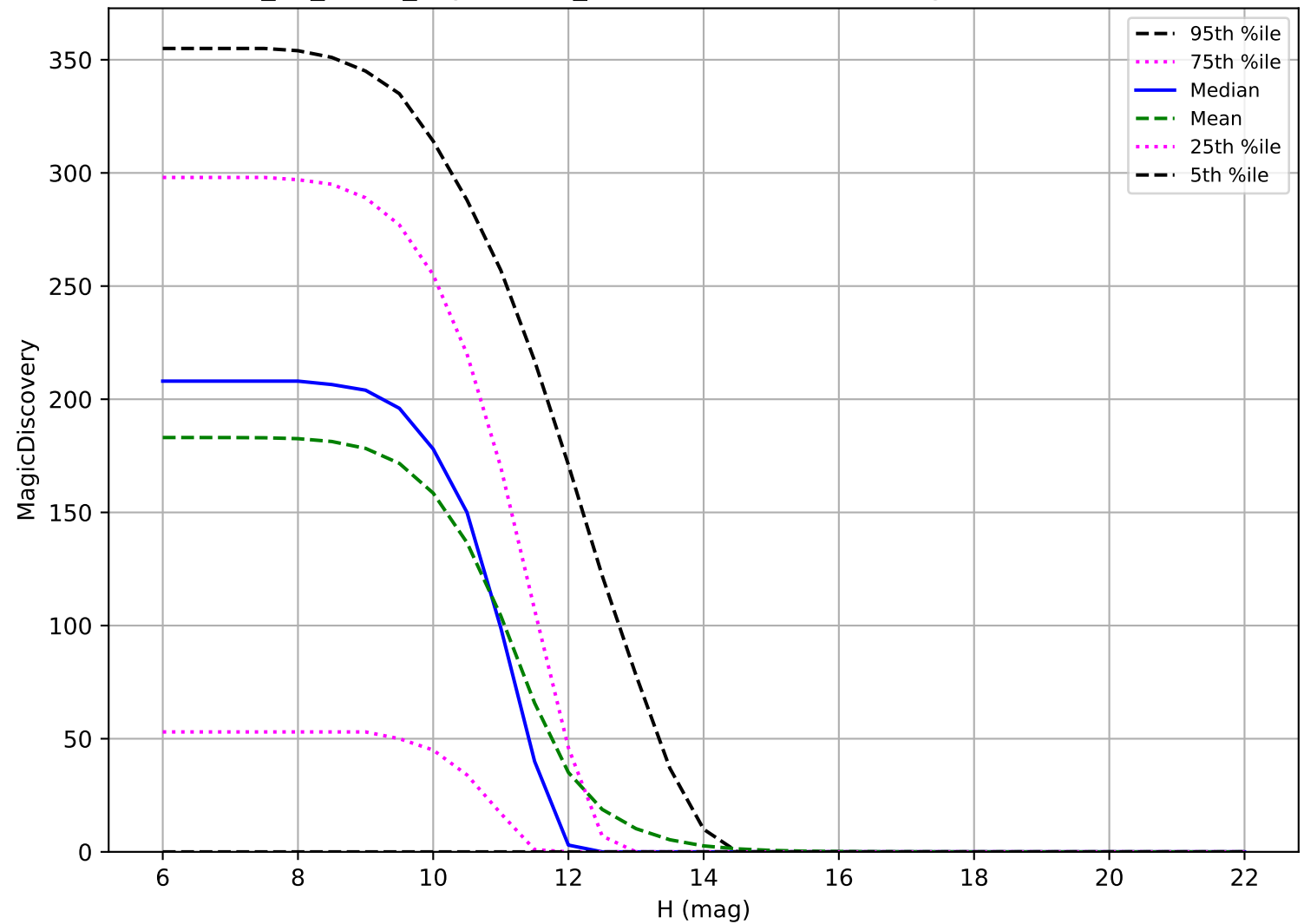
too_10_1v3.4_10yrs: OCC_r20 6 detections in 60 nights detection loss
