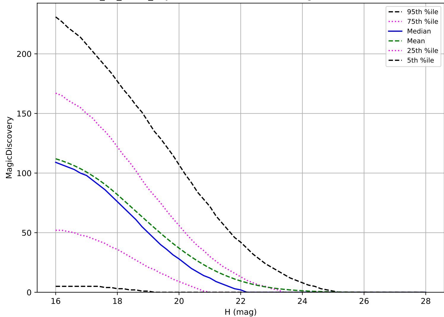
too_10_1v3.4_10yrs: NEO 6 detections in 60 nights detection loss
