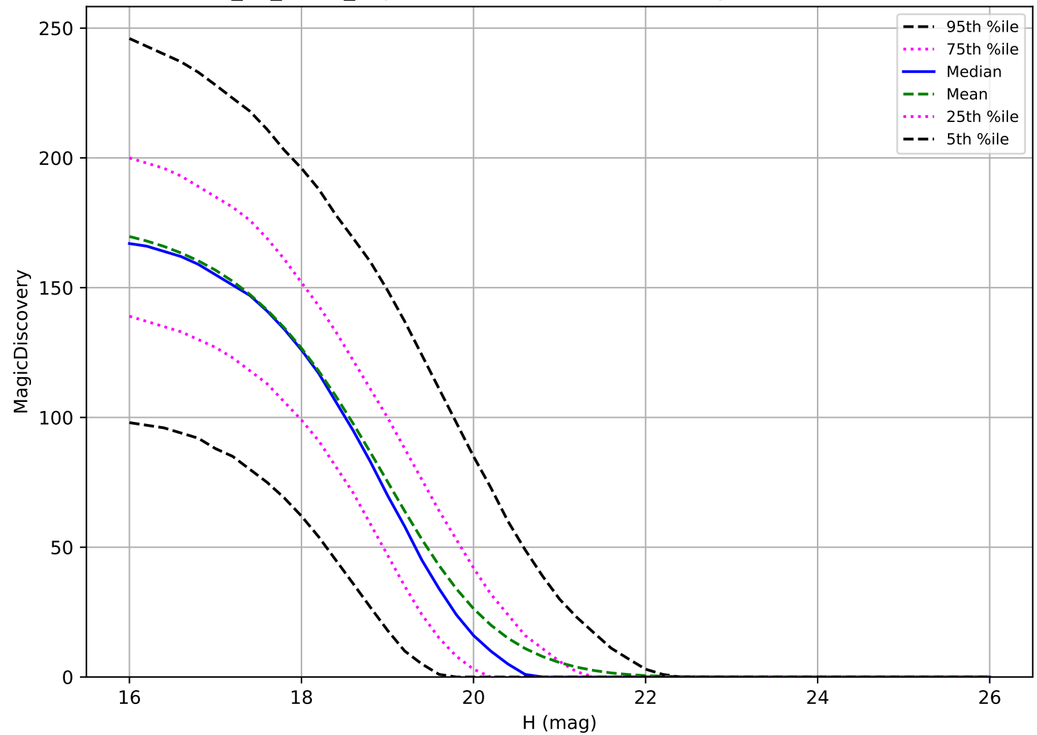
too_10_1v3.4_10yrs: MBA 6 detections in 60 nights detection loss
