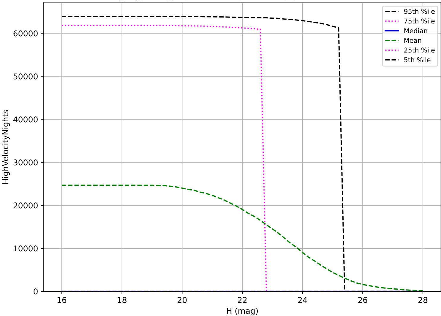
too_10_1v3.4_10yrs: PHA High velocity pair detection loss
