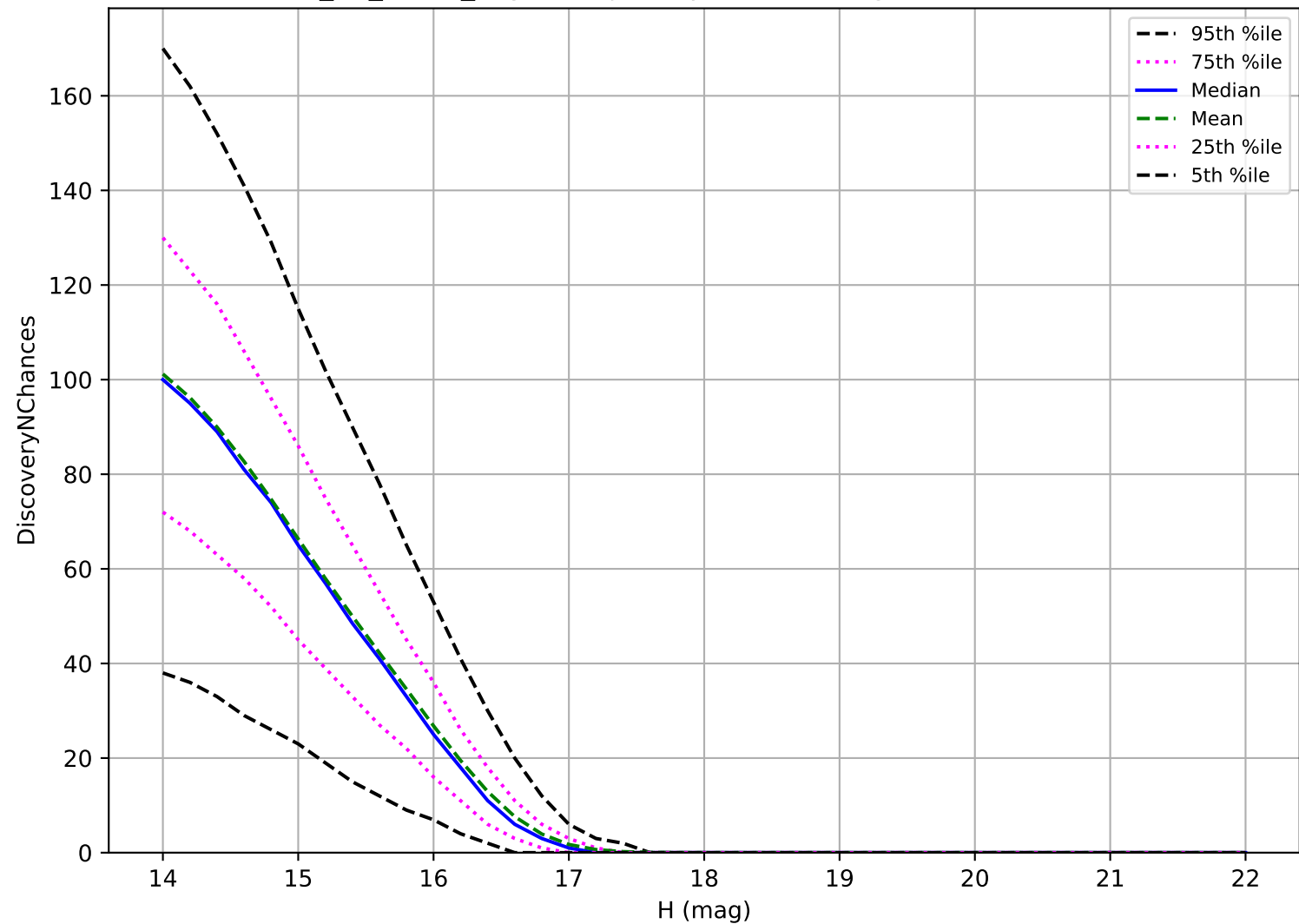
too_10_1v3.4_10yrs: Trojan 3 pairs in 15 nights detection loss
